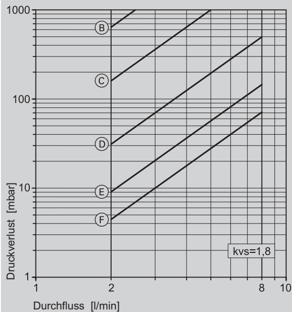
DN 15/2,0 - 8,0 l/mn
