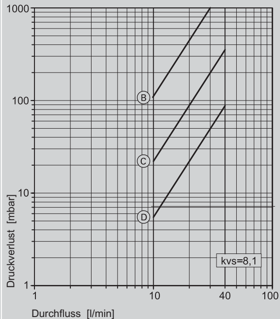
DN 25/10,0 - 40,0 l/mn
