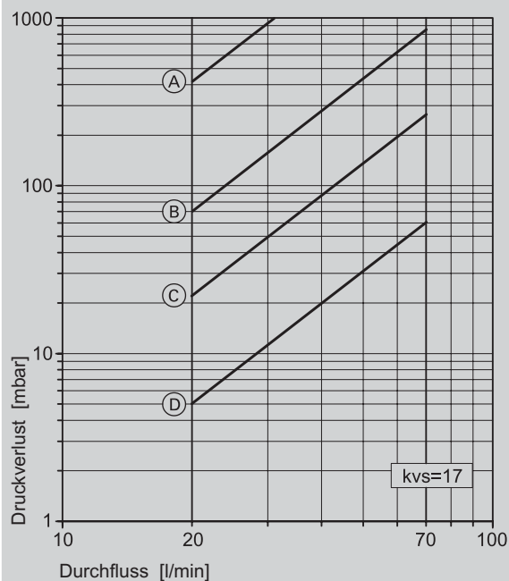
DN 32/20,0 - 70,0 l/mn
