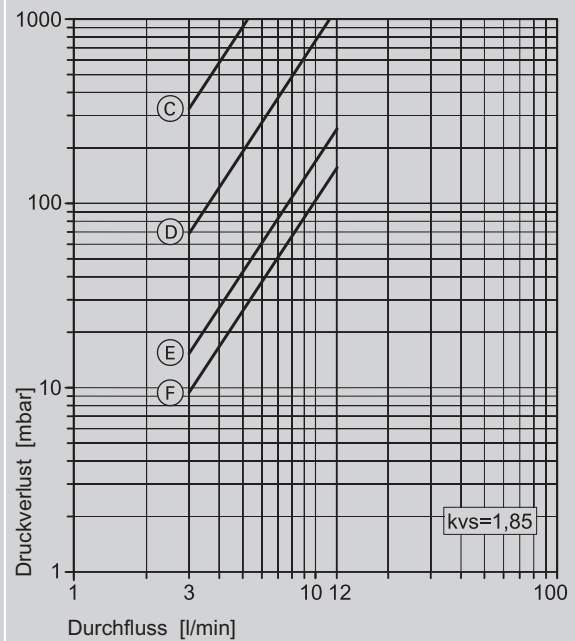
DN 15/3,0 - 12,0 l/mn
