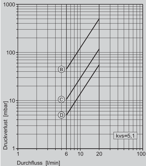
DN 25/6,0 - 20,0 l/mn
