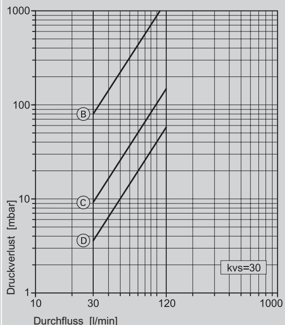
DN 40/30,0 - 120,0 l/mn
